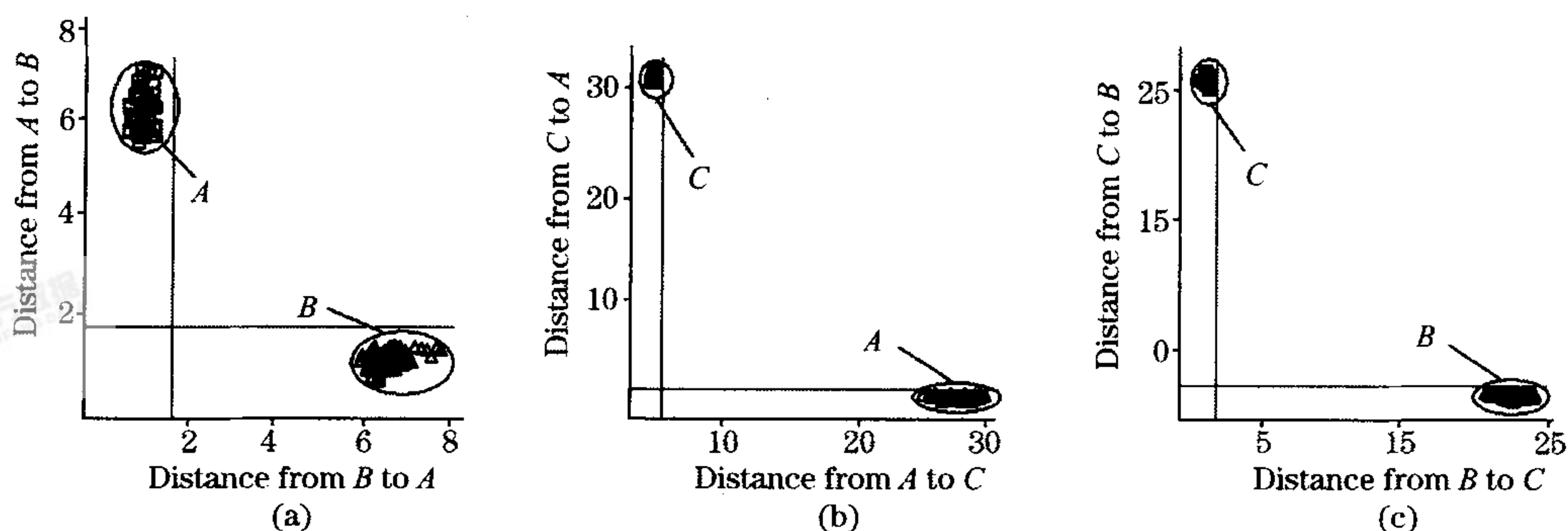
Fig. 2 Class plot of A, B and C from classification of principal component analysis-Mahalanobis distance
