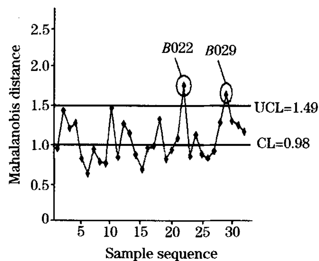
Fig. 3 3\sigma -control plot of Mahalanobis distance for B class
