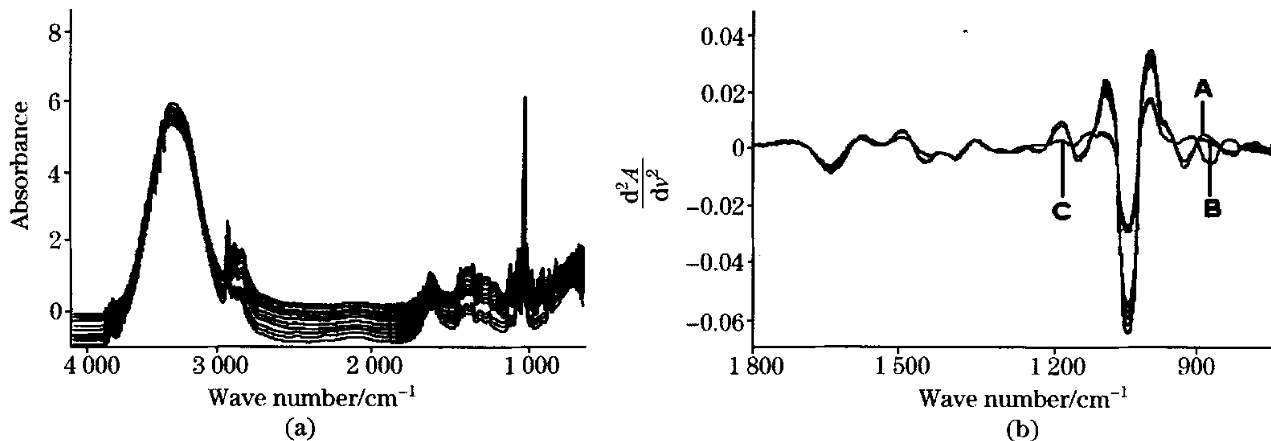
Fig. 1 FTIR-ATR spectra of tobacco flavour (a) and their 2nd derivative spectra(b)
